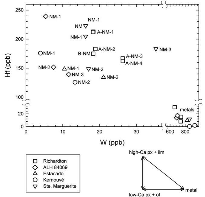
Fig. 4. Hf versus W contents for the different fractions of the analyzed H chondrites. Data for some of the NM (non-magnetic) fractions from Ste. Marguerite are from Kleine et al. (2002). The Hf and W concentrations in the coexisting phases of these H chondrites are not colinear, indicating that presence of at least three independent components for Hf and W among the coexisting phases. These components are high-Ca pyroxene+ilmenite, olivine+low-Ca pyroxene, and metal.
