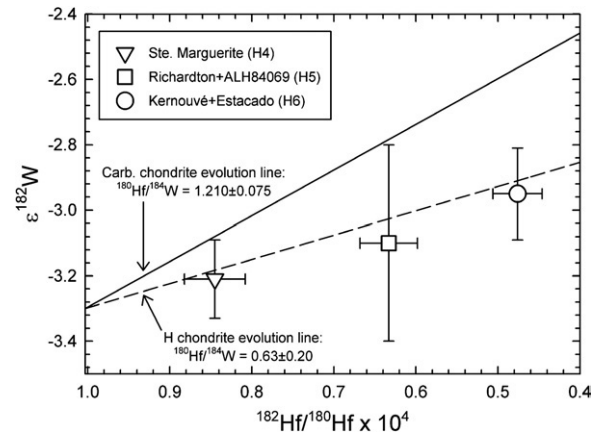
Fig. 8. W isotope evolution diagram for H chondrites. The carbonaceous chondrite evolution line is defined by their present-day \epsilon^{182}\text{W} and the initial \epsilon^{182}\text{W} of Allende CAIs. The analyzed H chondrites depart from the evolution line of carbonaceous chondrites, indicating evolution in a reservoir with a Hf/W ratio lower than that of carbonaceous chondrites.
