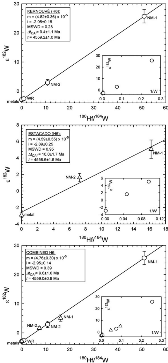
Fig. 3. \epsilon^{182}\text{W} versus ^{180}\text{Hf}/^{184}\text{W} for H6 chondrites Kernouvé and Estacado. m =initial ^{182}\text{Hf}/^{180}\text{Hf} , i =initial \epsilon^{182}\text{W} . Regressions are calculated using the model 1 of IsoPlot (Ludwig, 1991). Details regarding the calculation of ages are given in the text. \Delta t_{CAI} is the formation interval relative to CAIs; the absolute age t is calculated relative to the angrites D'Orbigny and Sahara 99555 (see text).
