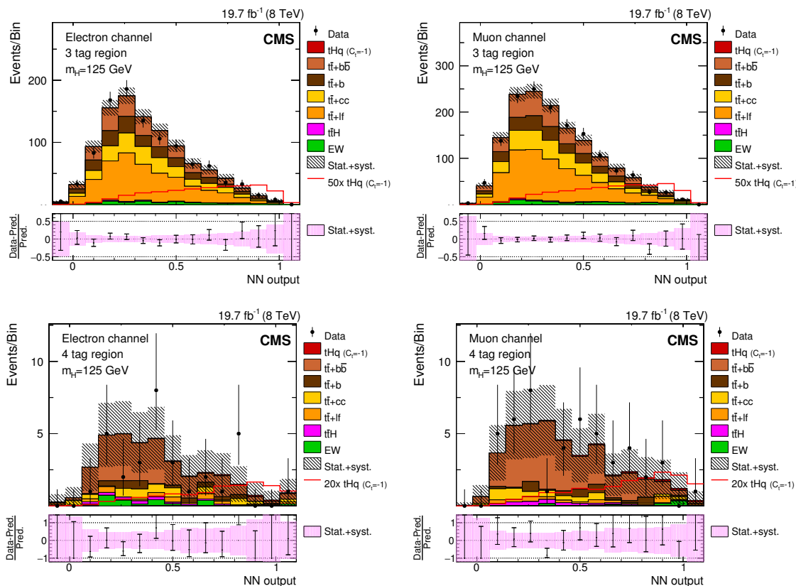
Figure 3. Distributions of the NN output for the H \rightarrow b\bar{b} channel for events with three (four) b-tagged jets are shown in the upper (lower) row. The left (right) column shows events containing a high- p_T electron (muon). All backgrounds are normalized to the output of a maximum likelihood fit of the corresponding distributions. “EW” indicates electroweak backgrounds: single top quark, W/Z boson plus jets, and di- and tri-boson production. The line shows the expected contribution from the tHq process with C_t = -1 multiplied by the factor indicated in the legend. In the box below each distribution, the ratio of the observed and predicted event yields is shown. The shaded band represents the post-fit systematic and statistical uncertainties.
