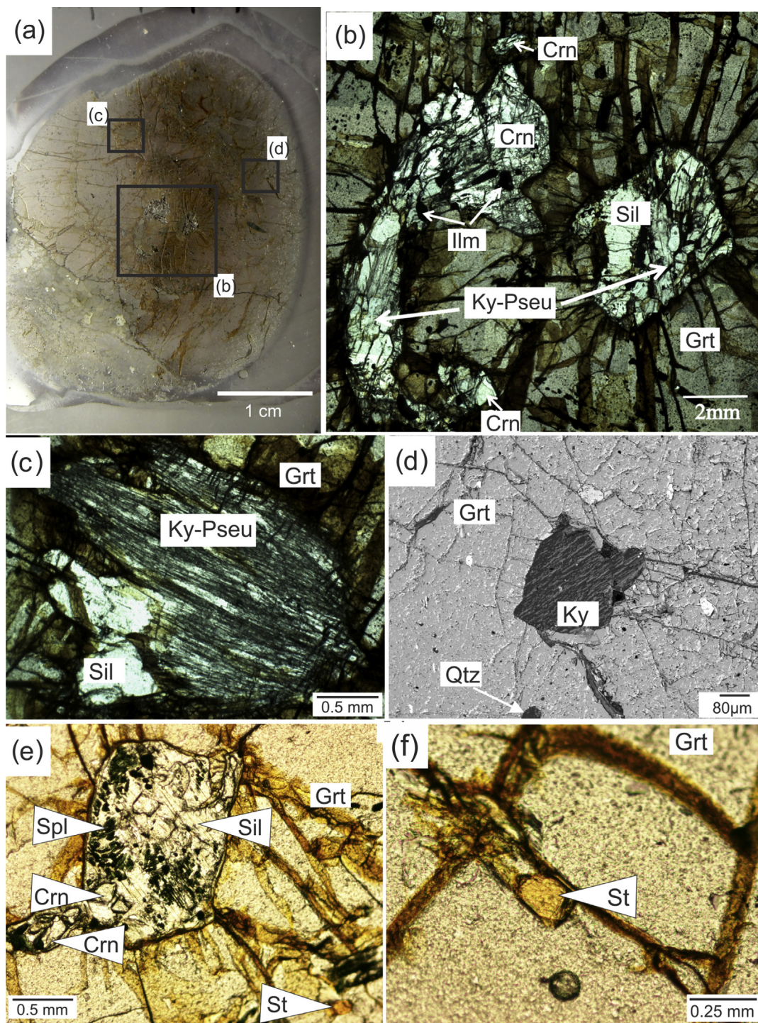
Figure 5. Petrography of Grt 4 in Rock D (images b–d show the textures of the Grt 4 of the image (a)); images i–m show the textures of the Grt 4 of the image (h)). (a) A petrographic thin section showing a Grt 4 (b) as a mosaic with anhedral corundum and sillimanite clusters which pseudomorph kyanite in the core area; (b) aggregate of fibrolitic sillimanite pseudomorphing kyanite; (c) isolated kyanite grain towards the rim are. An isolated quartz grain also present close to kyanite, (e) tiny spinel inclusions and corundum inclusions in coarse prismatic sillimanite; a staurolite grain is also present in the bottom right hand side of the image; (f) an isolated staurolite grain; (g) formation of pyrophyllite towards the rim; (h) petrographic thin section of another porphyroblastic garnet grain; (i) core existence of corundum and sillimanite clusters which pseudomorph kyanite in the mantle area; (j) tiny inclusion of quartz close to kyanite pseudomorph after sillimanite; (k) isolated cluster of sillimanite pseudomorphing kyanite; (l) close association of isolated quartz and cluster of sillimanite pseudomorphing kyanite; (m) isolated quartz, staurolite and cluster of sillimanite pseudomorphing kyanite.
