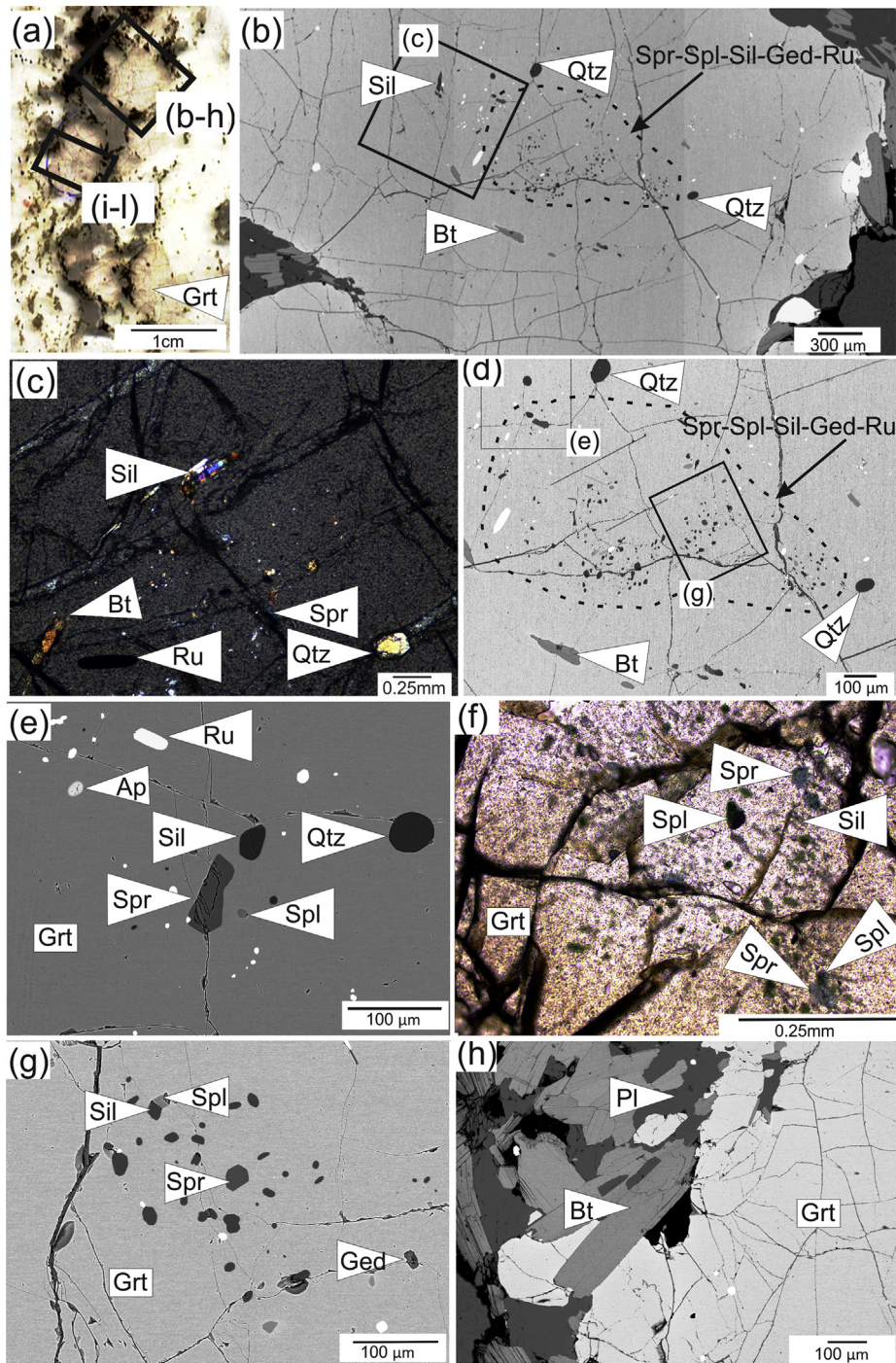
Figure 2. Microtextures of Grt 1 in Rock A (b–h): microtextures of the first Grt 1 grain shown in image (a) in garnet rich layer; i–l: microtextures of the second Grt 1 grain shown in the garnet rich layer; m–o: microtextures of the third Grt 1 grain shown in image (n) in the garnet rich layer. (a) A petrographic thin section representing the garnet rich layer; (b) a mosaic of BSE images of a Grt 1 in which the quartz-deficient core domain and quartz saturated mantle to rim domains are shown; (c) CPL image showing the inclusion phases at the boundary of silica-saturated and silica-deficient domains; (d) closer view of the core area of the garnet in image (c); (e) inclusions of sapphirine, spinel, silimanite and quartz; (f) tiny inclusion phases of garnet coexisting with sapphirine + spinel; (g) coexistence of spinel and sillimanite. Gedrite is also present, (h) formation of biotite + plagioclase corona around garnet; (i) a mosaic of rim of one side to rim of opposite side (cross the core) of a garnet; (j) the image representing the inclusion phases close to the boundary of silica-saturated and silica-deficient domains; (k) BSE image of core area of the garnet, spinel. Tiny sillimanite are also present, (l) closer view of the center part of the image (k) where coexistence of gedrite + sapphirine and gedrite + spinel are present; (m) presence of clusters of spinel-sapphirine-sillimanite toward the rim area of garnet; (n) a thin section representing the garnet of image (a) a mosaic of the garnet in which the rim area of one side contains a silica-deficient domain and the rest of the portion representing a silica saturated domain.
