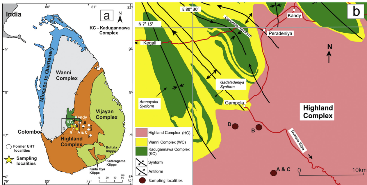
Figure 1. (a) Geological map of Sri Lanka showing the lithotectonic subdivision (after Cooray, 1994). A star shows sampling locality and circles show UHT localities reported so far: 1. Osanai (1989): T = 900 °C; 2 & 3. Kriegsman and Schumacher (1999): T = 830 °C (here it is corrected as 950 °C); 4. Sajeev and Osanai (2004a): T = 950 °C; 5. Sajeev and Osanai (2004b): T = 1150 °C; 6. Osanai et al. (2006): T = 1000 °C; 7. Sajeev et al. (2007): T = 925 °C; 8. Dharmapriya et al. (2015a): 950–975 °C. (b) Detailed geological map (modified after Kröner et al., 2003) and the sampling localities.
