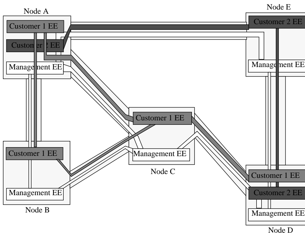
Figure 2: An active network with nodes A, ..., E, on which VANs for Customers 1 and 2 have been installed.
