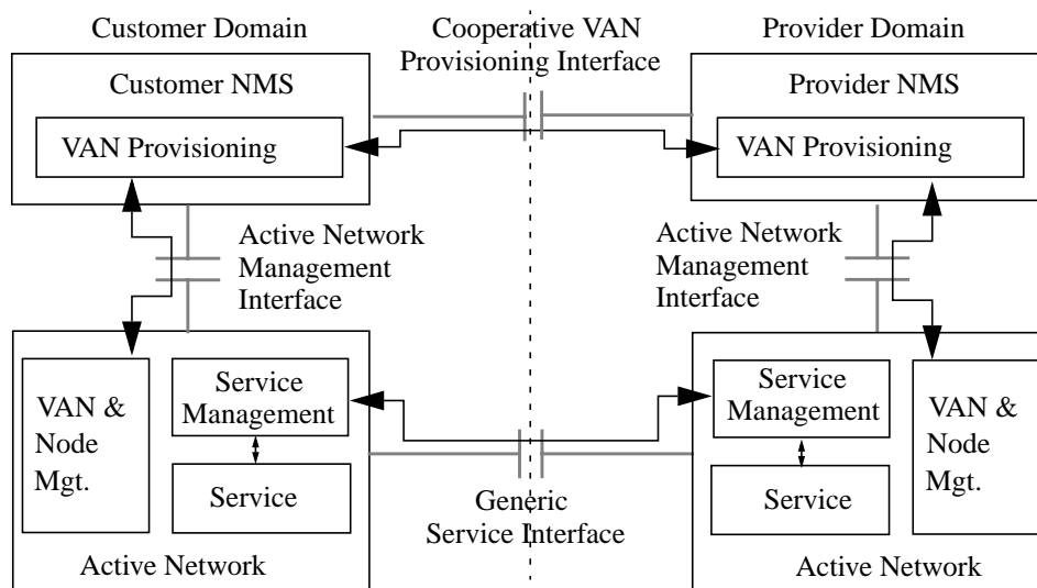
Figure 1: Customer-Provider Interaction in an Active Telecom Environment
