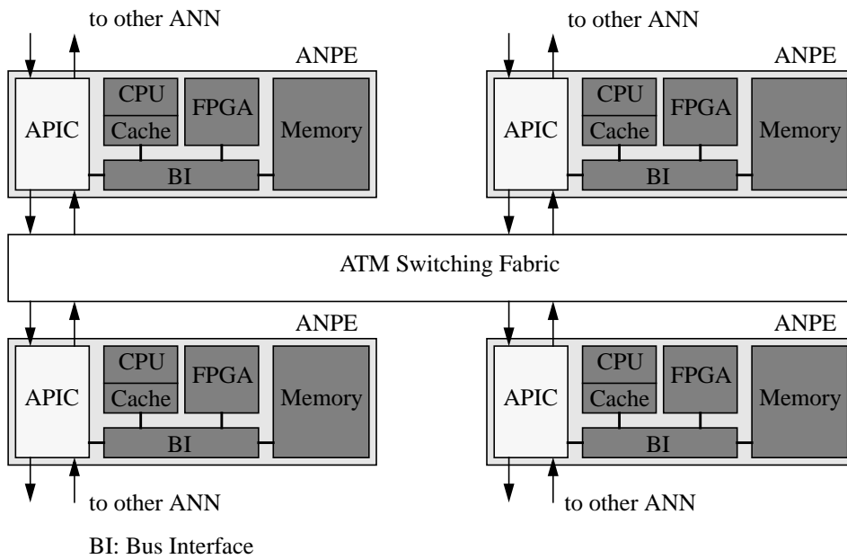
Figure 8: Hardware Architecture of an Active Network Node (ANN)
