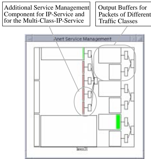
Figure 7: Node Structure after Installing an IP-Service and Upgrading to a Multi-Class-IP-Service
