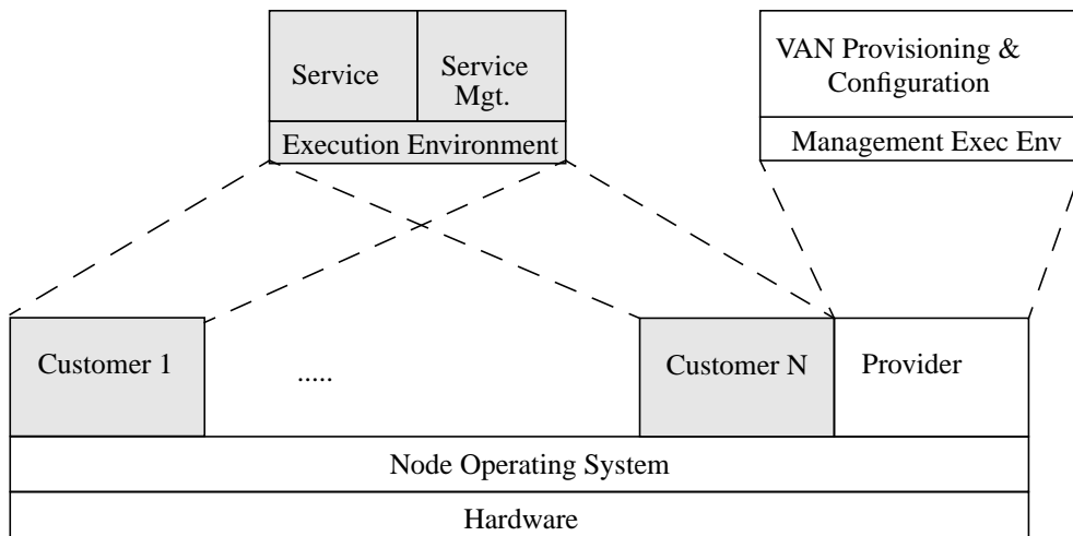
Figure 3: Architecture of an Active Network Node in a Telecom Environment
