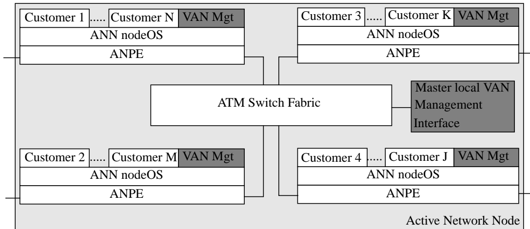
Figure 9: Design where an ANN node is seen as a single Active Network Node
