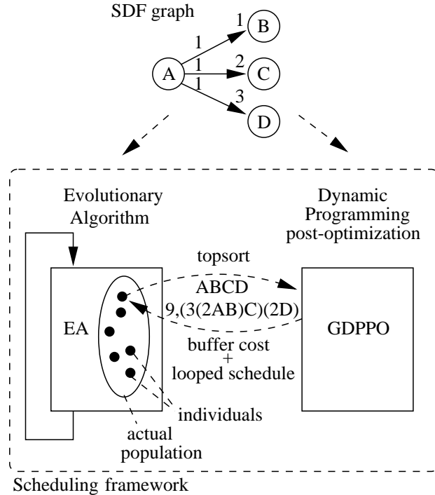
Figure 1.3: Overview of the scheduling framework using Evolutionary Algorithms and Dynamic Programming (GDPPPO: generalized dynamic programming post optimization for optimally parenthesizing actor orderings [MBL94], discussed further in Section 2.3.2) for constructing buffer memory optimal schedules.
