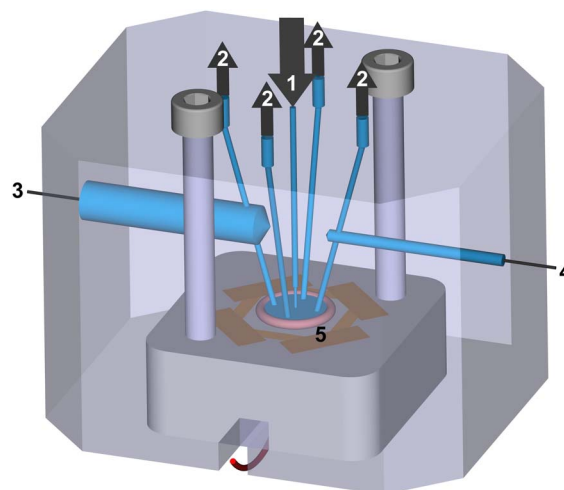
Figure 1. Sketch of the electrochemical flow cell. (1) Inflow from tube-in-tube (de)airation system, (2) outlets, (3) RE compartment, (4) CE compartment, (5) WE compartment with O-ring sealing and top-contact to copper plate. Dimensions are not to scale for clarity of presentation.
