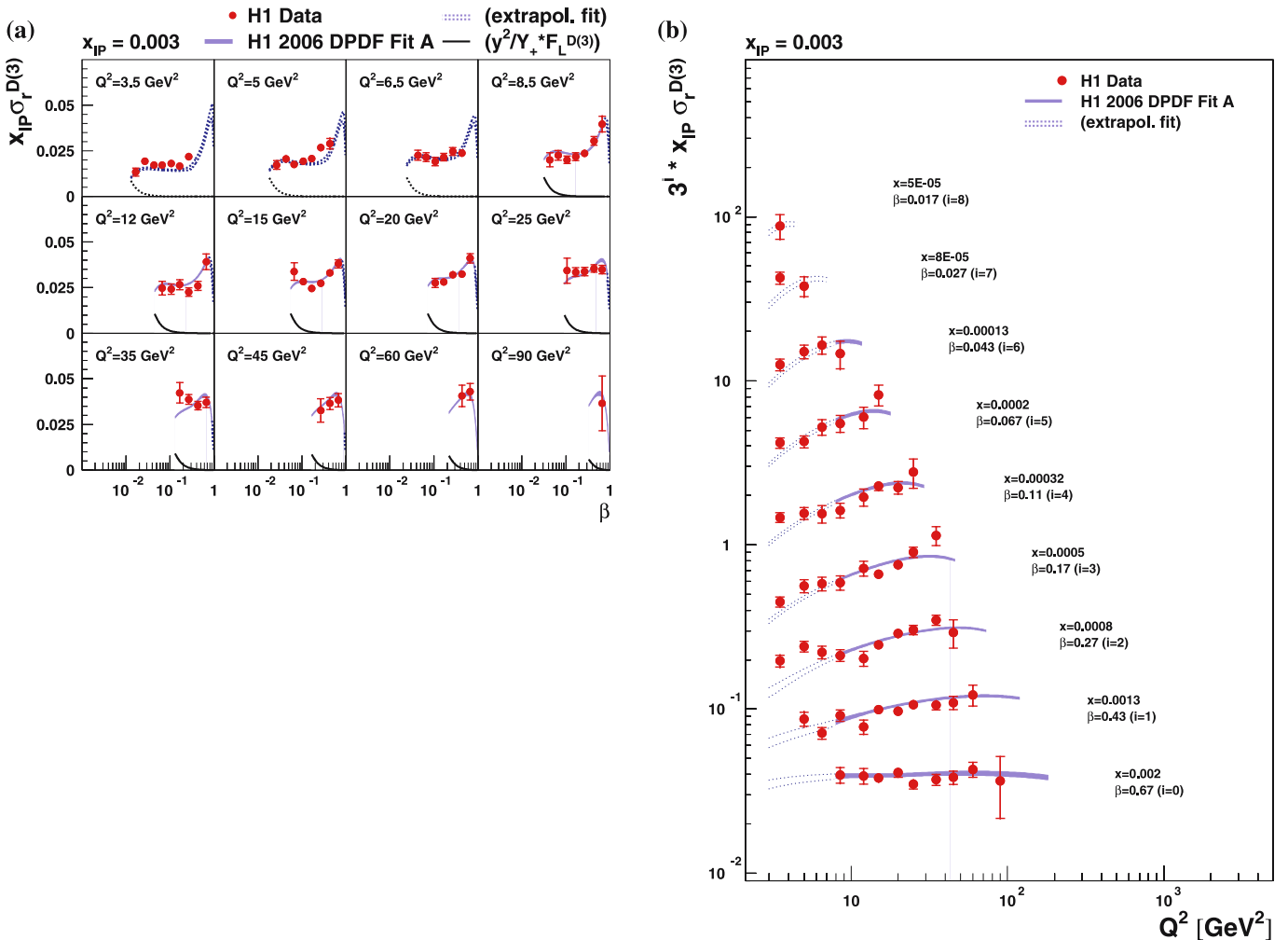
Fig. 4. The \beta and Q^2 dependences of the diffractive reduced cross section, multiplied by x_{IP} , at x_{IP} = 0.003 . In a, the quantity y^2/Y_+ \cdot F_L^D(3) is also shown, as extracted from the ‘H1 2006 DPDF Fit A’. Adding this quantity to the reduced cross section yields F_2^D(3) . See the caption of Fig. 2 for further details
