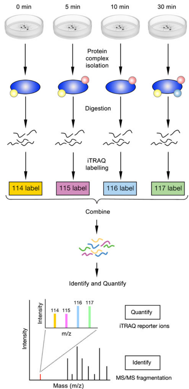
Fig. 5 Quantitative analysis of changes in protein complex stoichiometry using iTRAQ. Desired treatment of cells or extraction of tissue from different conditions is followed by isolation of protein complexes using affinity purification and proteolysis using trypsin. Isobaric iTRAQ tags are chemically added to the N terminus and lysines of every peptide and samples from different times or conditions are labelled with a different iTRAQ tag (4 shown, up to 8 possible), and then combined. Samples can then be analysed via ESI- or MALDI-MS. MS/MS analysis of iTRAQ labelled samples generates a spectrum that yields the sequence of the peptide, and iTRAQ reporter ions ( red peak : expanded in close-up), which can be seen in the low mass range (114–121 m/z ). Comparison of the peak intensities for each reporter ion allows quantitation. In the example shown, iTRAQ analysis would allow the elucidation of changes in the proteins attached to the bait protein (shown as a blue oval ) over time
