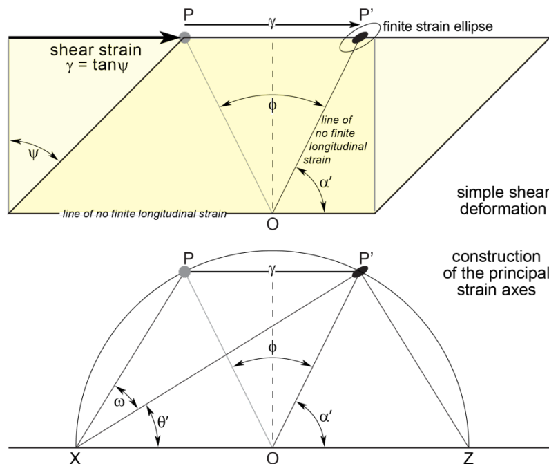
Relationship between the orientation of a shear foliation (X axis in 2D) with respect to the shear plane (i.e. shear zone boundary)
