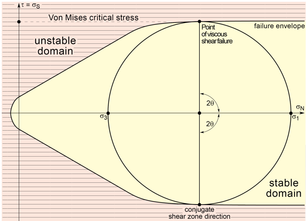
Orientation of new shear zones fitting the Von Mises criterion in a Mohr diagram
