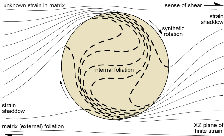
Helical trails of inclusions in a garnet porphyroblast rotated by 180° String-cylinder model of Schoneveld 1977 Tectonophysics 39(1-3) 453-471
