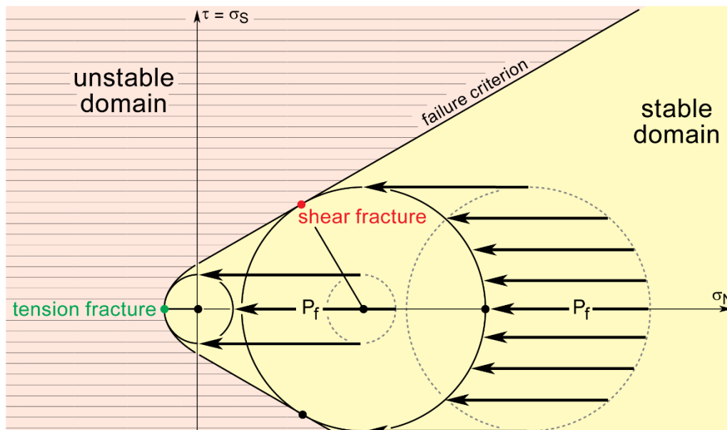
Effect of the differential stress on the fracture type in two-dimensional Mohr diagram
