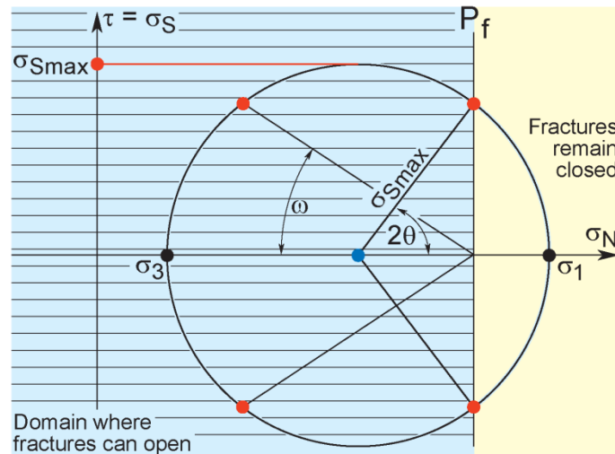
Delimitation of fracture dilation domains in function of pore fluid pressure P_f in two-dimensional Mohr diagram
