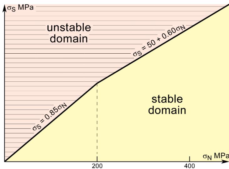
Byerlee’s law for pre-existing fault surfaces
