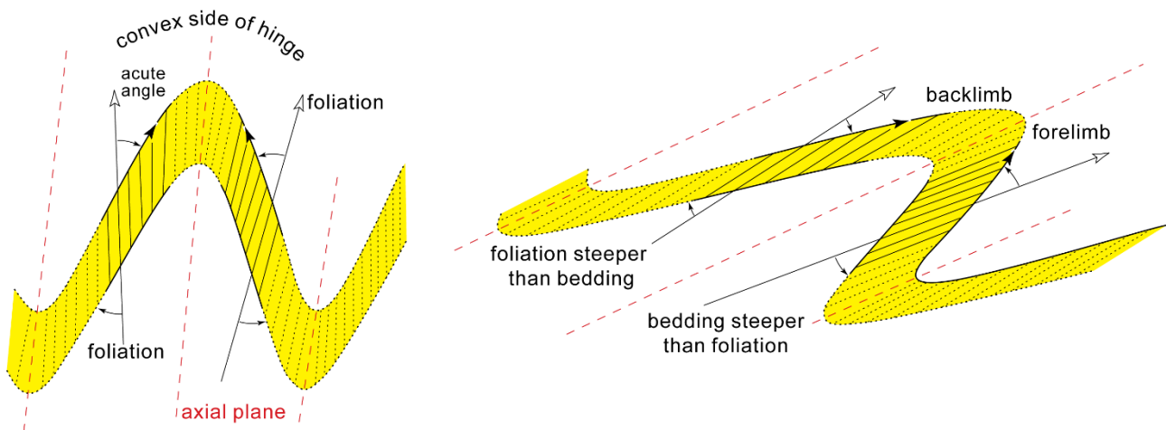
Angle relationship between bedding and foliation in fold profiles
