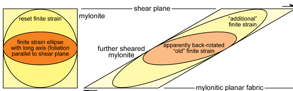
Instability of the finite strain ellipsoid in mylonites once the plane of maximum flattening (foliation) is parallel to the shear plane
