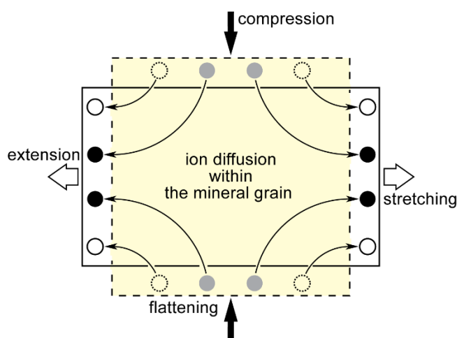
Change in shape of a grain due to diffusion-controlled mass transfer
