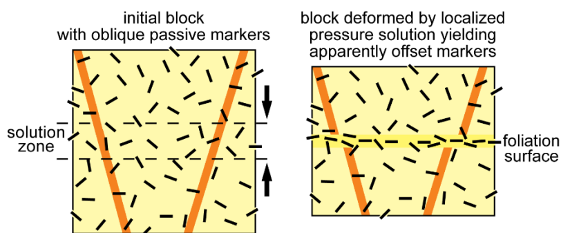
Reorientation of platy minerals due to removal of their matrix by solution
