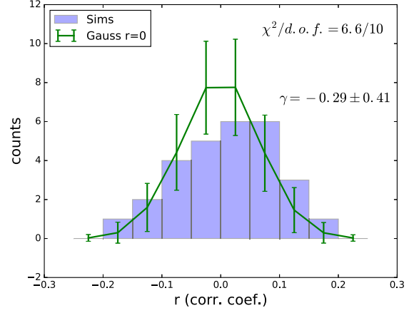
Figure 4. Distribution of correlation coefficients of \alpha (see the text) between different mask rotations for the HALOGEN mock catalogues (‘Sims’). We compare it to the expected distribution of correlations if \alpha followed a Gaussian distribution and results from different masks were uncorrelated (‘Gauss r=0 ’). We find that this hypothesis (with no free parameter) to be compatible with our simulations. We also find that the observed skewness in the distribution \gamma is within the expected statistical noise level under the same hypothesis.
