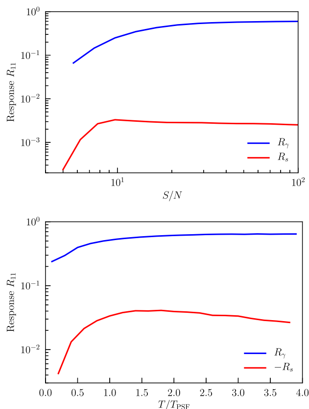
Figure F1. Variation of the 1–1 components of the selection bias response correction R_s and mean calibration response R_\gamma with signal-to-noise (top) and galaxy size relative to PSF size (bottom).
