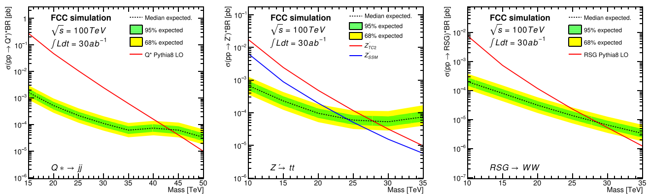
Fig. 15.7 Sensitivity to various resonance models using fully hadronic final states. For left to right: excited quarks Q^* in the dijet channel; Z' in the \bar{t}\bar{t} hadronic channel (SSM and top-assisted technicolour [389], TC2, models); G_{RS} in the WW fully hadronic channel. From Ref. [383]
