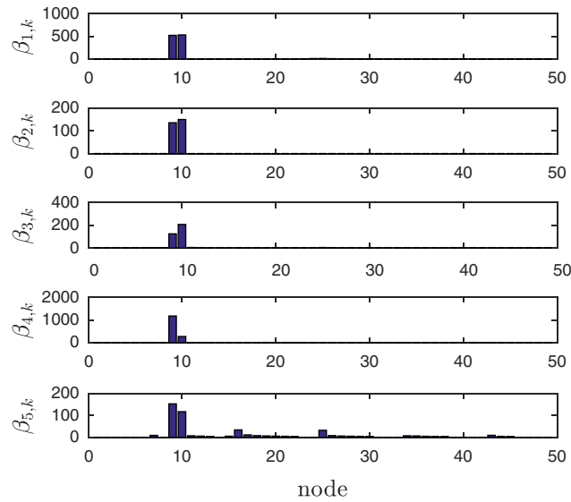
FIGURE 8 Diagnostics stage: damage index for 15% damage in Bar element 10 (Case study I)
