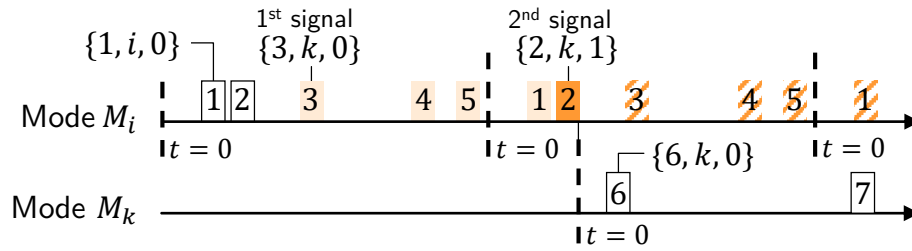
Figure 5.9 Example of mode change from mode M_i to M_k . The dashed lines show the start of the mode hyperperiods. Each numbered box represents a communication round with its id . The content of some of the host beacons is shown next to the corresponding rounds. In r_3 , the host sends the first signal to change to mode M_k . During this transition phase, the rounds are lightly colored. In the dark colored round, the host sets TB = 1 . This is the second signal – directly after this round, mode M_k starts executing. Dashed rounds are not executed.
