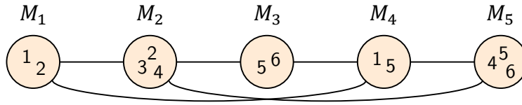
Figure 5.7 The mode graph \mathbb{M} discussed in Examples 5.1 and 5.2. Five modes are represented by circles, the possible transitions between modes as arcs. Six applications a_1 to a_6 are specified. The specification is shown with the numbers in the circles; e.g., S_1 = \{a_1, a_2\} . Mode M_i has priority i .
