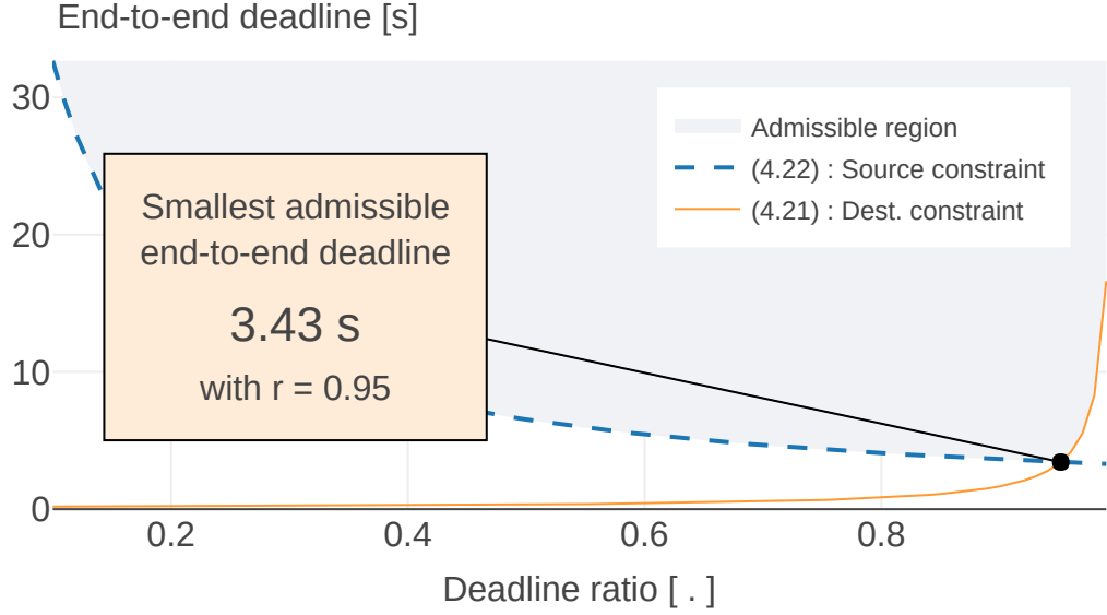
Figure 4.10 The smallest admissible end-to-end deadline for C_{net} = 1 s and T_{f,min}^d = 0.1 s is D_{min} = 3.43 s. Equations (4.21) and (4.22) each define a feasible region for (r, D) tuples. The intersection defines the admissible region.
