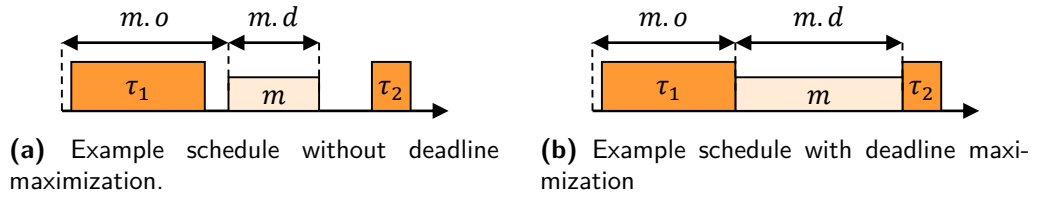
Figure 5.6 Illustration of the impact of the message deadlines maximization. If Figure 5.6a is a valid schedule, then Figure 5.6b is also valid, but it relaxes the constraints on other modes which also contain message m . Maximizing the message deadlines improves the schedulability of the multi-mode problem (Section 5.5).
