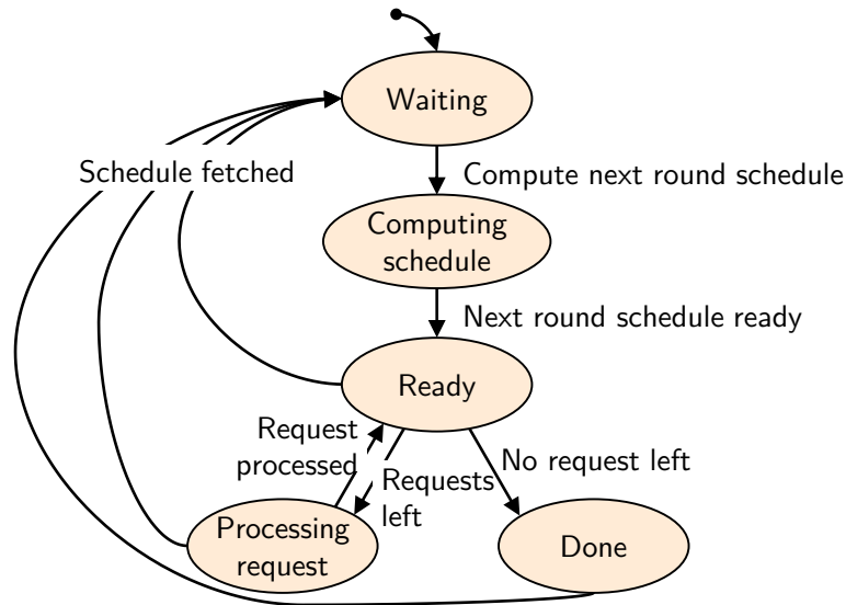
Figure 4.8 State-machine of the host AP . AP first computes a valid schedule for the next round. Then, the AP processes queued DRP requests, one at a time, and recomputes a (new) schedule accounting for the newly admitted flow.
