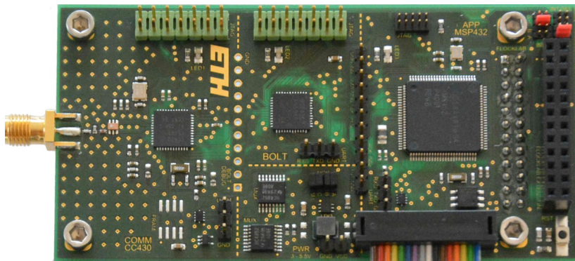
Figure 1.7 Integrated design of the same DPP as in Figure 1.5, featuring a TI MSP432 [182] as application processor (right) and a TI CC430 SoC [181] as communication processor (left). Bolt sits in the middle, implemented on a TI MSP430 core featuring 64k FRAM [183].
