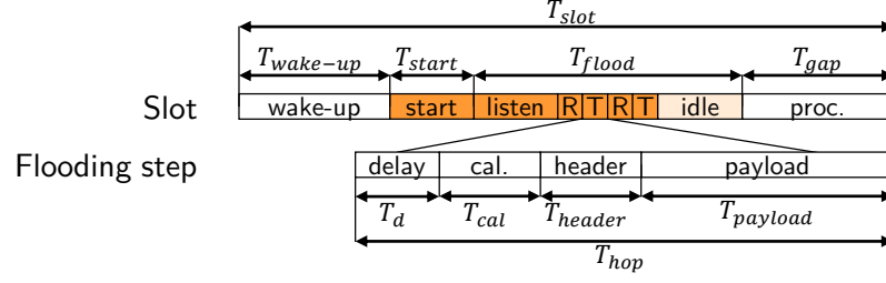
Figure 5.13 Break-down of a communication round. At the slot level, the colored boxes identify phases where the radio is on. In the “idle” phase, the radio is turned off in practice, but this idle time depends on each node’s distance to the initiator. To estimate the energy saving of rounds (Figure 5.15), we assume that the radio stays on for the whole time of T_{flood} , as specified in Equation (5.40).
