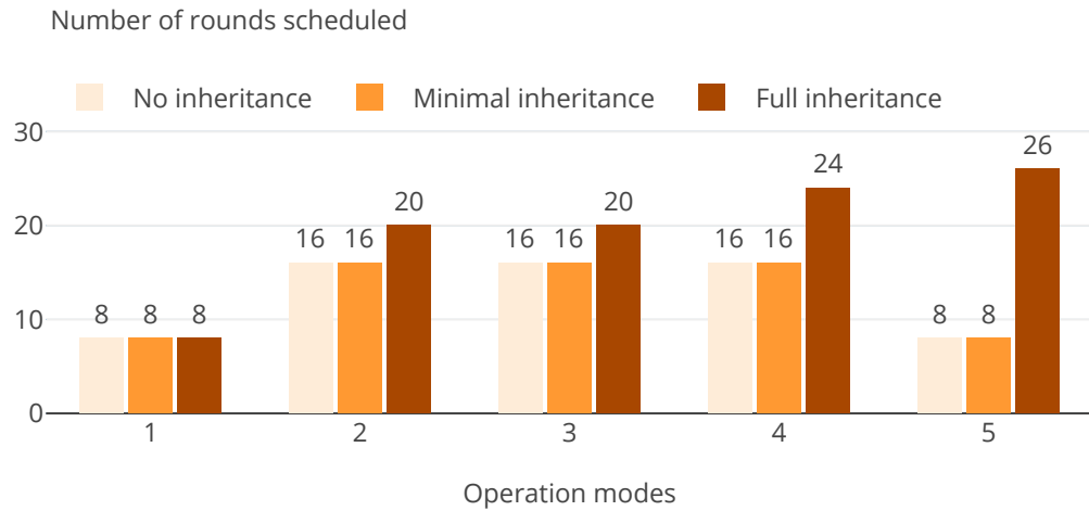
Figure 5.11 Number of rounds in the different modes' schedule, depending on the inheritance approach considered. We consider the number of rounds scheduled over 80s, which is the least common multiple of the modes' hyperperiod.
