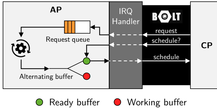
Figure 4.9 Request queue and alternating buffer on the host AP . Incoming messages from CP trigger an interrupt and are handled immediately. DRP requests are put in a dedicated queue for later processing (Figure 4.8). When CP writes a schedule request, the interrupt handler fetches the most recent schedule from the “Ready buffer” and write it to Bolt.
