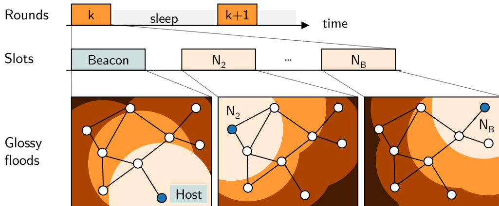
Figure 5.3 The TTnet network stack. TTnet organizes communication in time-triggered rounds, between which nodes turn their radio off to save energy. The rounds are composed of (up to) B communication slots preceded by a beacon, sent by the host to distribute runtime control information. In each slot, an one-to-all communication is realized using Glossy [74].
