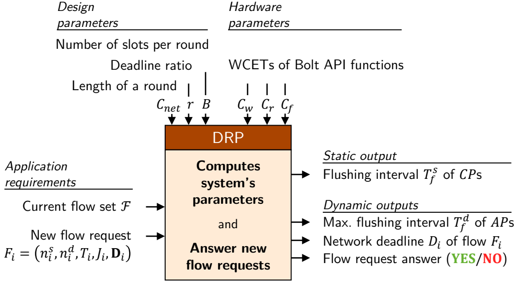
Figure 4.6 Inputs and outputs of DRP . Hardware and design parameters are fixed at design time, while the application requirements may change at runtime. DRP statically computes the flushing interval of CPs; all other outputs are dynamically computed whenever the flow set \mathcal{F} changes.
