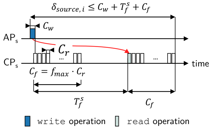
Figure 4.13 Worst-case analysis of the source delay. A packet is written as early as possible such that it misses a flush and must wait until the next one.
