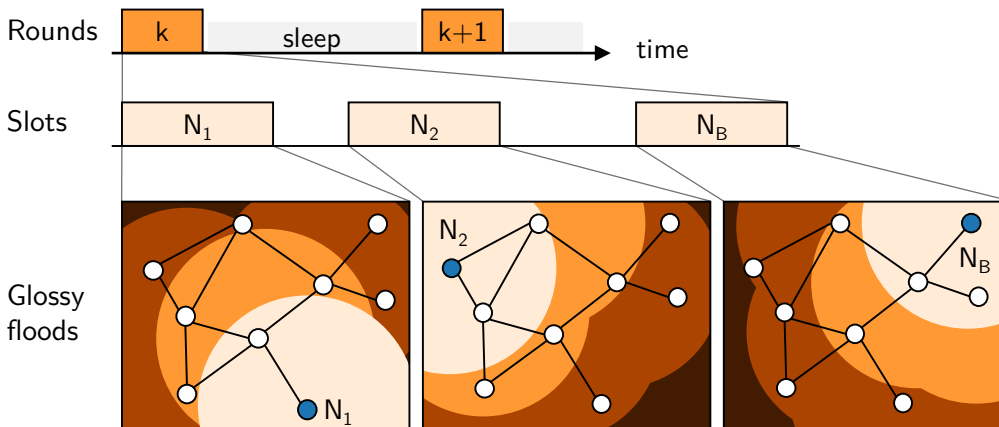
Figure 1.4 Thanks to synchronous-transmissions based flooding, a multi-hop network can be abstracted and scheduled like a shared bus. Communication is organized in rounds, composed of time slots; in each time slot, a node initiates a flood which allows to send a message to any other node(s) in bounded time. This mimics the operation of classical field bus, but with a wireless design.
