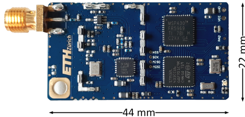
Figure 1.9 A different DPP2 “communication board” featuring a STM32L4 ARM core and Semtech latest generation long-range low-power LoRa transceiver with up to +22 dB m transmit power at 868 MHz (Semtech SX1262) [164].
