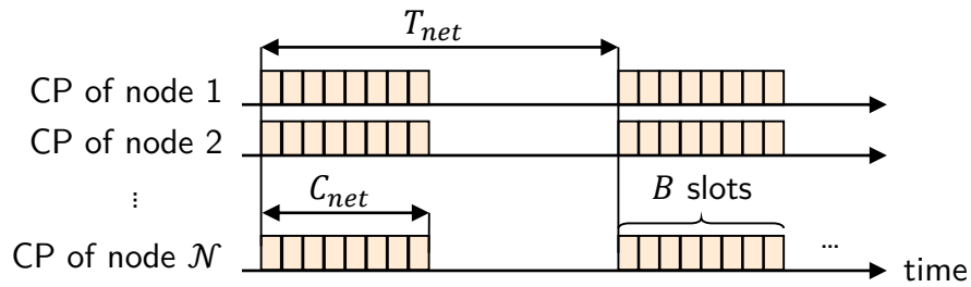
Figure 4.4 Operations in Blink are globally time-triggered. Communication occurs in rounds of equal duration C_{net} . Each round consists of a sequence of up to B_{max} exclusive time slots, each of which serves to send one message using Glossy floods [74]. The time interval between two consecutive rounds ( T_{net} ) may vary. During a round, the CP of all nodes in the system participate in the flood.
