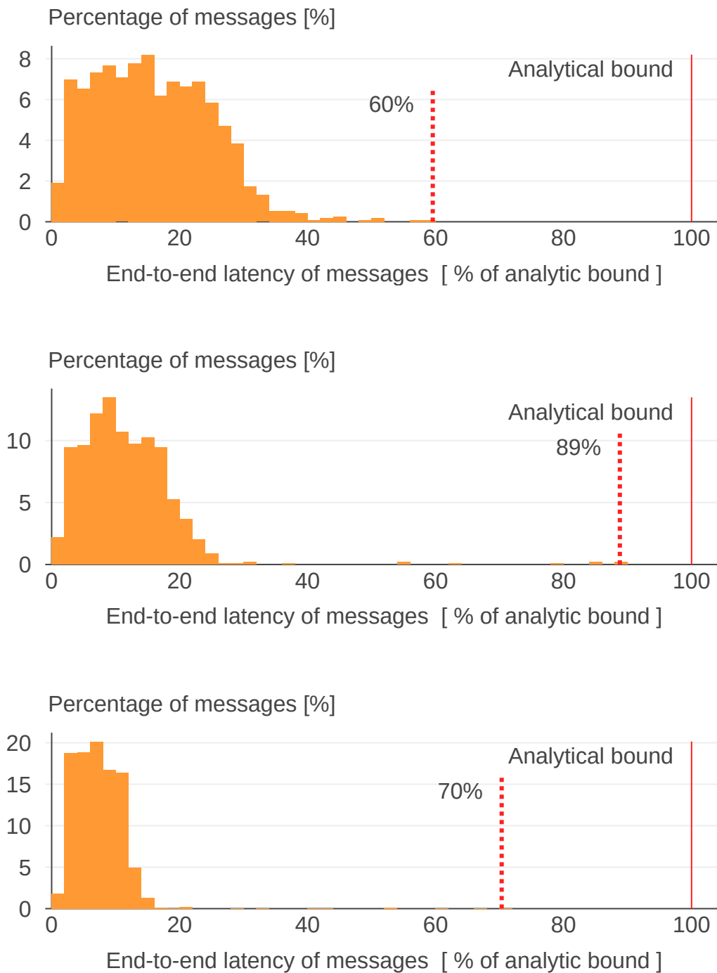
Figure 4.12 Distribution of end-to-end latency of messages, shown as percentage of the analytical worst-case latency for a DRP run using different flow sets (Table 4.3). Top – Low utilization. Middle – Medium utilization. Bottom – High utilization.
