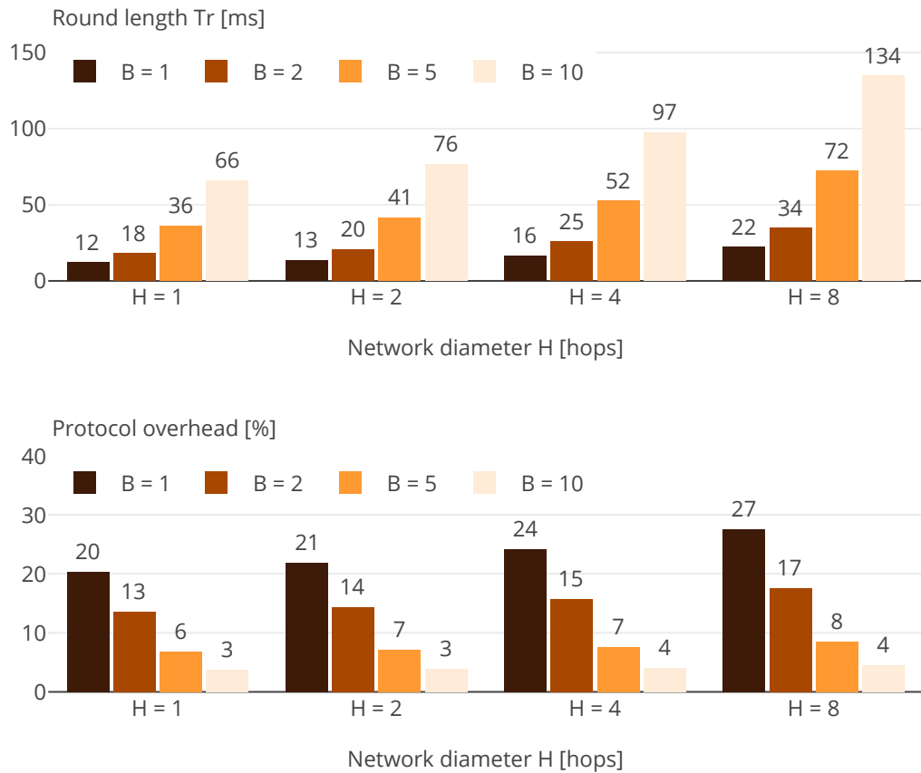
Figure 5.14 Example values of round length (top) and protocol overhead (bottom) computed using the TTnet model (Section 5.9.2). The protocol overhead is computed as the percentage of time spent to send the beacons relative to the overall communication time for a round containing B slots. Payload is set to 16 bytes and we use N = 2 transmissions in the Glossy floods [74].
