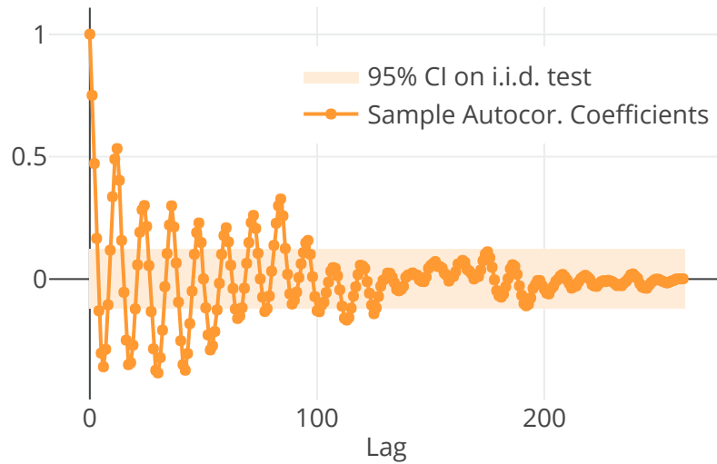
Figure 2.5 Autocorrelation plot for the wireless link quality on FlockLab, based on the raw data collected by the testbed maintainers [100] (data from August 2019). The dataset contains one test every two hours. The first peak at lag 12 (i.e., 24h) reveals the daily seasonal component. The data also show another at lag 84; which corresponds to one week. Indeed, there is less interference in the weekends than on weekdays: this creates a weekly seasonal component.
