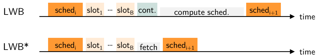
Figure 4.7 The original LWB (Top) and the modified round used in DRP (Bottom). DRP removes the contention slots, made redundant by the presence of dedicated control flows. Furthermore, the time span before sending the next round's schedule can be significantly reduced: indeed in DRP , the host CP can quickly fetch the schedule from the AP , which has done the computation in parallel.
