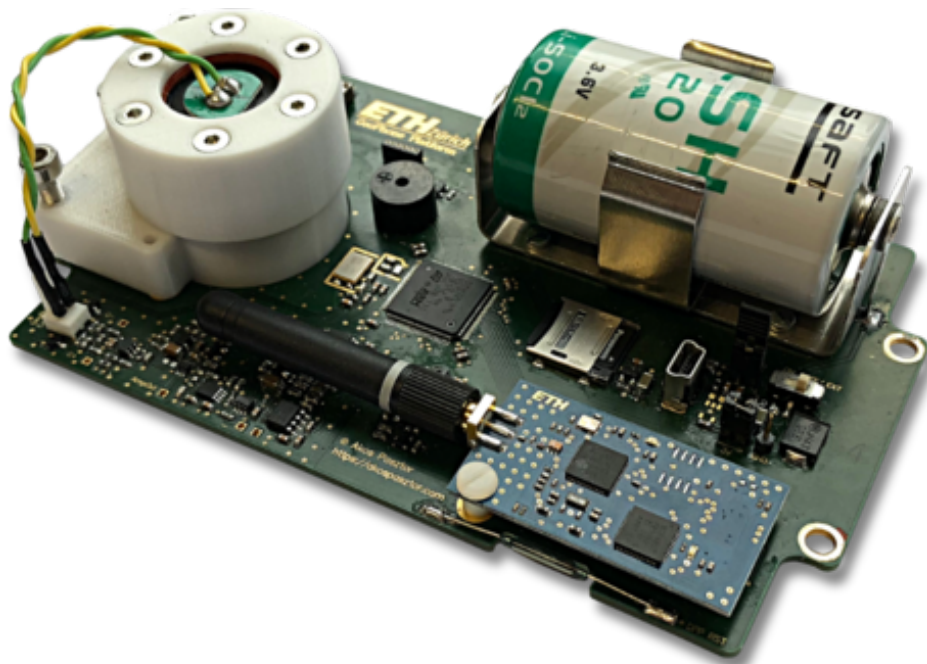
Figure 1.10 Battery-powered geophone sensor node based on the DPP2 design. The lower “application development board” includes a geophone sensor, an analog low-power threshold-based wake-up circuit, and an ARM-Cortex M4 [22] as application processor. On top sits the same “communication board” as in Figure 1.8. This design is currently deployed on the Hörnligrat of the Matterhorn [129].
