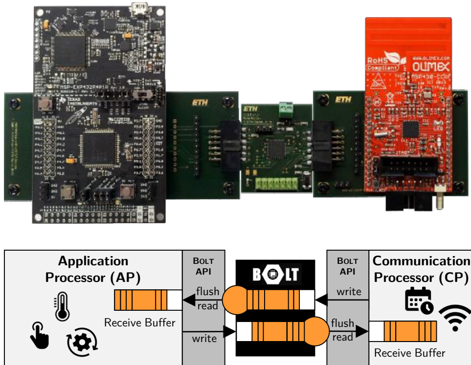
Figure 1.5 Top: Example of a custom-built heterogeneous DPP. Bolt (in the middle) interconnects a powerful application processor (TI MSP432 [182]) on the left with a state-of-the-art communication processor (TI CC430 [181]) on the right. Bottom: Conceptual view of the Bolt processor interconnect. Using the Bolt's API functions (write, read, and flush), the processors dedicated to application (AP) and communication (CP) can asynchronously exchange messages with predictable latency, while otherwise executing independently from one another.
