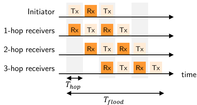
Figure 1.3 Glossy operation in a 3-hop network with 2 transmissions per node ( N )
