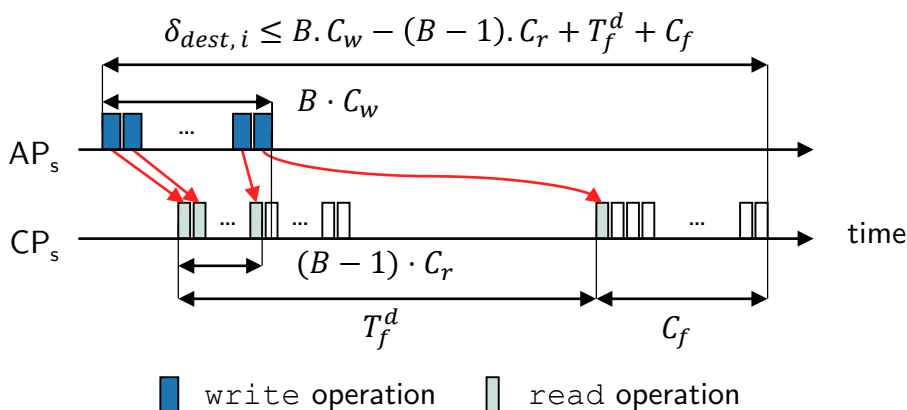
Figure 4.16 Worst-case analysis of the destination delay. A packet is written as early as possible such that it misses a flush and must wait until the next one.
