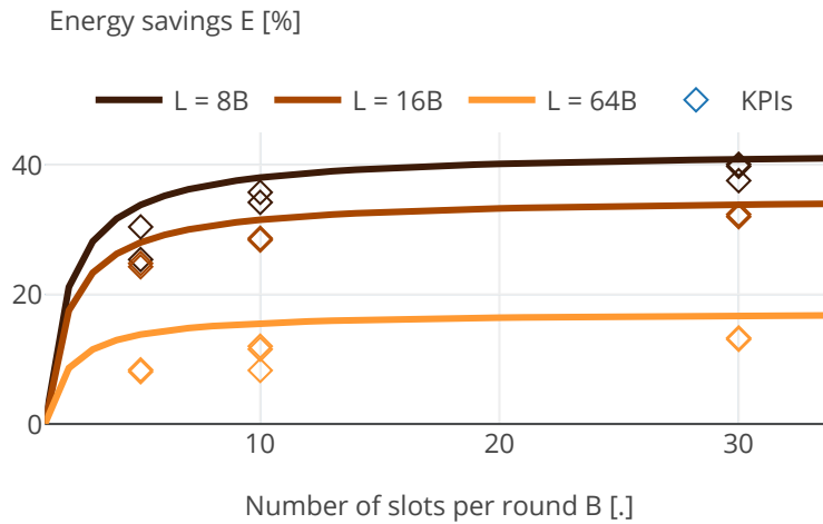
Figure 5.15 Relative radio-on time savings by using rounds compared to single messages. The energy savings induced by a round-based design grow with the number of number of slots per round (X-axis). Conversely, these savings become less significant as the payload size increases (lighter colors). The diamonds show our evaluation KPIs and thus estimate, with a probability of 95%, the average energy savings expected in 95% of the test runs. H = 4 , N = 2 .
