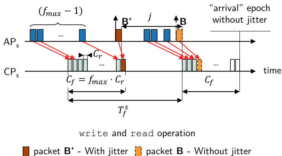
Figure 4.15 Influence of jitter on the network delay. Let us have a closer look at packet B from the previous figure, positioned as early as possible (i.e., if it were earlier, so would be A , which would then not miss its slot in round 1). Due to jitter, B is released earlier, say by a amount j . This can yield packet B' ( B with jitter) to be read out in a previous flush operation. In the worst-case, packet B' is read out one operation earlier as soon as j is bigger than T_f^s - C_f + C_r , which increases the mismatch m by T_f^s . Similarly, m increases by k \cdot T_f^s when j reached k \cdot T_f^s - C_f + C_r , which yields k = \left\lfloor \frac{j + C_f - C_r}{T_f^s} \right\rfloor and concludes to equation (4.29).
