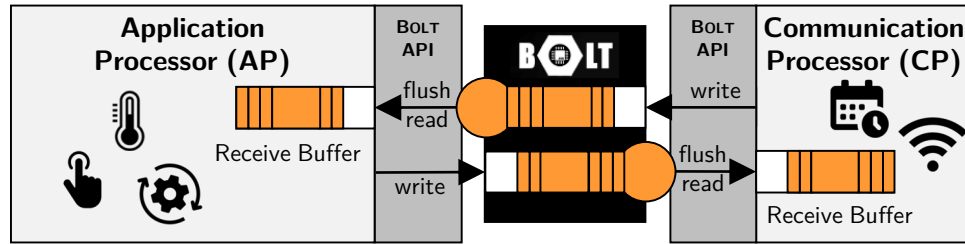
Figure 4.3 Conceptual view of the DPP, based on the Bolt processor interconnect. Using functions write , read , and flush , the application ( AP ) and communication ( CP ) processors can asynchronously exchange messages with predictable latency. The AP executes application tasks (e.g., sensing, actuation, control, etc.) while the CP is dedicated to radio communication.
