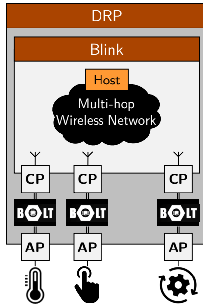
Figure 4.2 System model of the Distributed Real-time Protocol ( DRP ). A set \mathcal{N} of DPP nodes are forming a wireless CPS . The communication processors ( CPs ) run the Blink real-time protocol [209] to exchange messages across a multi-hop wireless network. The CPs forward and receive messages from their application processors ( APs ) through Bolt [175]. DRP is a global scheduler that arbitrates end-to-end communications between the APs . On each AP , the application tasks can be scheduled freely (e.g., using a polling server, rate monotonic, etc.) as long as the resulting schedule satisfies the DRP contracts (Section 4.4). The host is a (logically) global network manager which arbitrates the access to the shared wireless medium; i.e., it runs the Blink and DRP schedulers. Physically, one of the nodes plays the role of the host.
