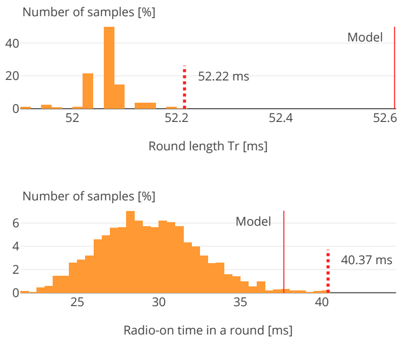
Figure 5.16 Distributions of round length (top) and radio-on time (bottom) measurements from all the nodes, collected in one series of 60 runs (Serie 2, L = 16 , B = 5 ). While the distribution of round length is very narrow, the radio-on time exhibits a much larger spread. We can see that the TTnet model provides a generally overestimate the radio-on time, which is expected since it assumes that nodes keep their radio on for the entirety of T_{flood} (Equation (5.40)), which is not the case in practice: nodes turn the radio off when they have transmitted a packet N times.
