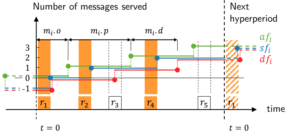
Figure 5.5 Representation of arrival, demand, and service functions of message m_i . The lower part shows the five round, r_1 to r_5 , scheduled for the hyperperiod. m_i is allocated a slot in the colored rounds, i.e., r_1 , r_2 , and r_4 . The allocation of m_i to r_3 instead of r_2 would be invalid, as r_3 does not finish before the message deadline, i.e., it violates (C2) . However, the allocation of m_i to r_5 instead of r_1 would be valid and result in r_0.B_i = 0 .
