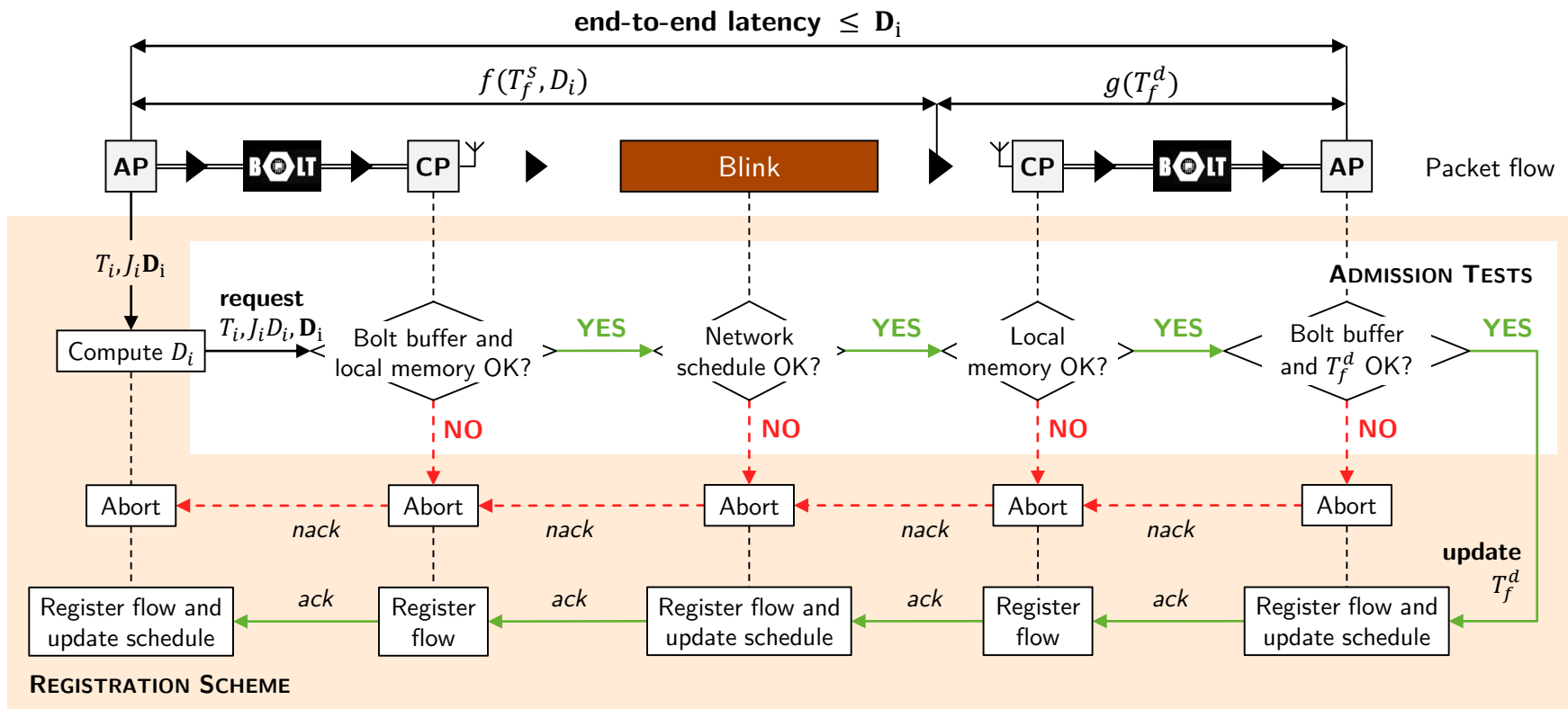
Figure 4.5 Steps and components involved when registering a new flow in DRP. Given a request for a new flow F_i = (n_i^s, n_i^d, T_i, J_i, D_i) , the source application running on AP_s at node n_i^s computes the flow's network deadline D_i . Then, all components check one after the other using specific admission tests whether they can admit the new flow. DRP registers a new flow only if all admission tests succeed, which eventually triggers changes in the runtime operation (the schedule) of Blink as well as of the source and destination application processors AP_s and AP_d .
