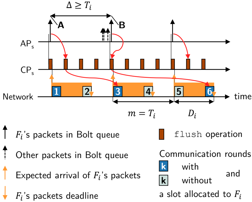
Figure 4.14 Worst-case analysis of the network delay without jitter. Because of the Bolt queue being empty, packet A misses the first flush operation (similarly as in Figure 4.13), hence the slot allocated to F_i in round 1 is wasted. Due to packets released from other flows in the meantime, packet B is flushed directly in the operation preceding round 3 , in which flow F_i is allocated a new slot. However, as packet A is still in queue, packet B is not served right away but is delayed until the next allocated slot (i.e., in round 6 ). This creates a mismatch of T_i for packet B . Furthermore, the mismatch cannot get bigger; assume B were to be available at CP_s earlier (i.e., one flush operation before, at least), because the time interval between A and B must be at least T_i , A would arrive earlier as well. Hence, A would not miss the slot in round 1 , B would be served in round 3 , and thus it would yield a smaller mismatch for packet B .
