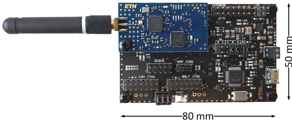
Figure 1.8 Redesign of the DPP concept into two separated boards, called the DPP2 [35]. The lower board (black), called “application development board” hosts the application processor (in this case, a TI MSP432 [182]) as well as all the I/O, power management, debugging, and other support functions. The upper board (blue) is called the “communication board” and hosts the communication processor (in this case, a TI CC430 SoC [181]) and the Bolt interconnect. This platform has been used for a prototype wireless CPS presented in [124, 123] and discussed further in Chapter 5.
