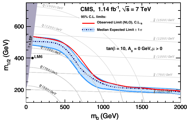
FIG. 4 (color online). Observed and expected 95% C.L. exclusion contours in the CMSSM (m_0, m_{1/2}) plane ( \tan\beta = 10 , A_0 = 0 , \mu > 0 ) using NLO signal cross sections with the C.L._s method. The expected limit is shown with its 68% C.L. range. The SUSY benchmark model LM6 is also shown.
