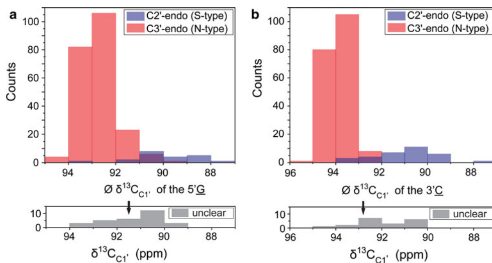
Fig. 6 Dependence of ^{13}\text{C} chemical shifts on the sugar pucker. Histograms showing the correlation between RNA C1' ^{13}\text{C} chemical shifts of (a) purines and (b) pyrimidines with the sugar pucker conformation. Riboses adopting C3'-endo conformation are colored red; riboses adopting C2'-endo conformation are colored blue. Riboses with unclear sugar pucker conformation are colored grey. Average values found for the \delta^{13}\text{C}_{\text{C1}'} of the 5'G and the \delta^{13}\text{C}_{\text{C1}'} of the 3'C are indicated by black arrows
