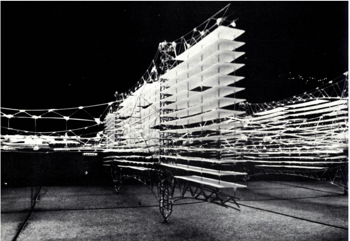
Figure 6. Takis Ch. Zenetos, physical model for the "Suspended city" ("Ville suspendue"), 1961. Image courtesy of the Takis Ch. Zenetos Archive.
