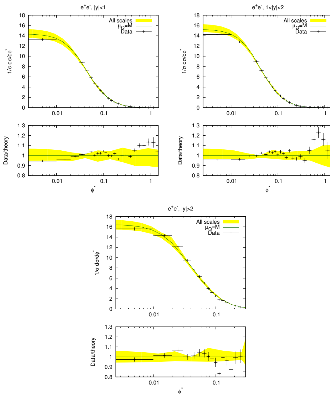
Figure 4. Comparison of the theoretical prediction NNLL+NLO for the \phi^* distribution to the experimental data collected by the DØ collaboration in the case of electrons, in three different vector boson rapidity bins, |y| < 1 , on the top left, 1 < |y| < 2 on the top right and |y| > 2 at the bottom.
