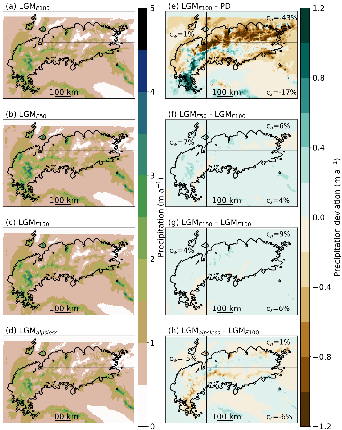
Figure B.9: Annual mean precipitation of the LGM E100 (a), LGM E50 (b), LGM E150 (c), and LGM alpsless (d) WRF climate datasets of Velasquez et al. (2020) and Velasquez and Raible (in prep). Precipitation deviation relative to the PD or the LGM E100 data are given in (e)–(h). The black outline indicates the geomorphologically reconstructed maximum ice extent of the LGM of Ehlers et al. (2011). The domain is divided into three sectors: a western, a north-eastern and a southern sector (black lines). c_w , c_n , and c_s indicate the relative change in precipitation inside the formerly glaciated area for the corresponding sectors.
