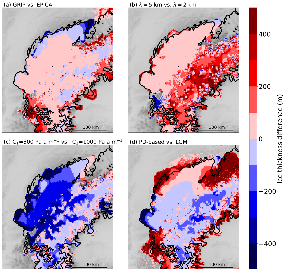
Figure 4.5: Deviation in maximum ice thickness relative to the reference simulation for the GRIP simulation (a), the \lambda = 5 km simulation (b), the C_1 = 300 \text{ Pa a m}^{-1} simulation (c), and the PD-based simulation (d). The black outlines indicate the geomorphologically reconstructed maximum ice extent (Ehlers et al., 2011).
