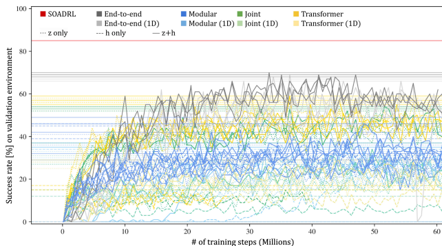
Fig. 8. 3 training sessions were performed for each of the two end-to-end and 18 NavRep architectures to account for the influence of network initialization on the results (legend as in Fig. 7). Horizontal lines mark the maximum success rate of each curve. The SOADRL success rate allows for comparison with methods that use exact human locations as input.
