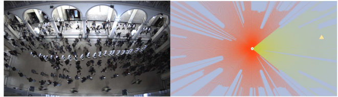
Fig. 1. Timelapse of an example target environment for autonomous navigation, snapshot of the corresponding LiDAR measurements on the right
