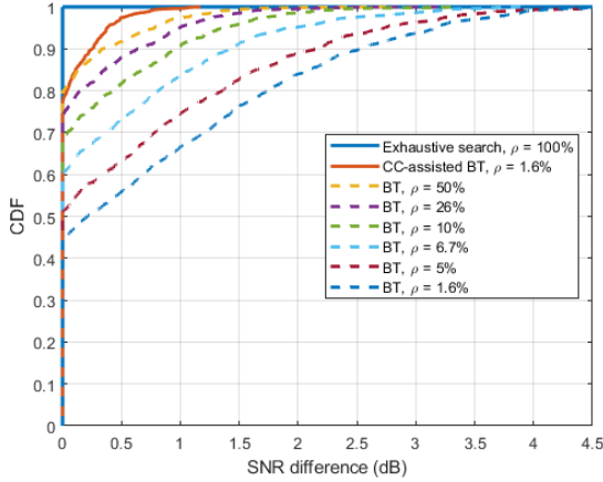
Fig. 4: The CDF of SNR prediction error in dB for beam tracking and CC-assisted beam tracking approaches. For beam tracking different refreshing criteria are considered. The CC-assisted beam tracking approach outperforms beam tracking approach with different refreshing frequencies.
