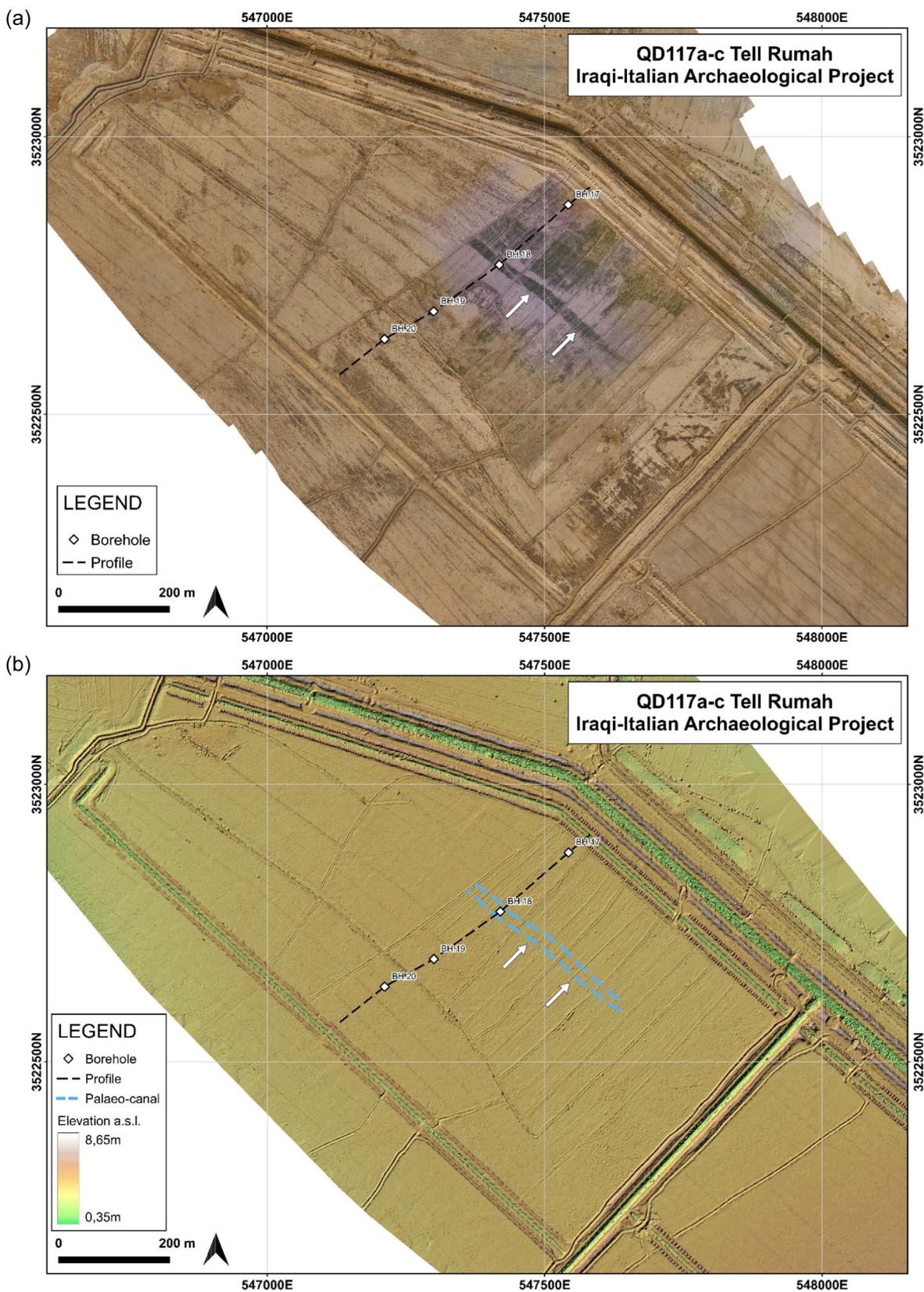
FIGURE 4 Tell Rumah (second half of fourth millennium B.C.E.), location of boreholes and profile, with white arrows indicating the artificial canal (data acquisition and processing by the QADIS project): (a) on the unmanned aerial vehicle (UAV) image 2017; (b) on the UAV image-derived digital elevation model.
