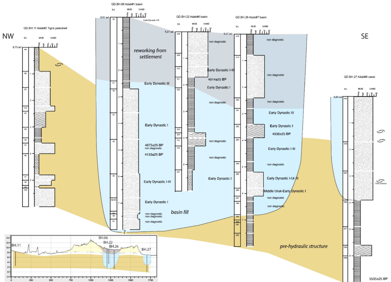
FIGURE 13 Adab/Bismaya (third millennium B.C.E.): Correlation between the five boreholes, with the indication of the stratigraphic units, the occurrence of radiocarbon and ceramic dating and the main interpretations: settlement, prehydraulic structure substrate, canal and harbour filling, with possible reworked material on the top. In the inset, the boreholes are projected on a high-resolution topographic profile, to show the real geometry ( x = distance as m; y = elevation as masl).
