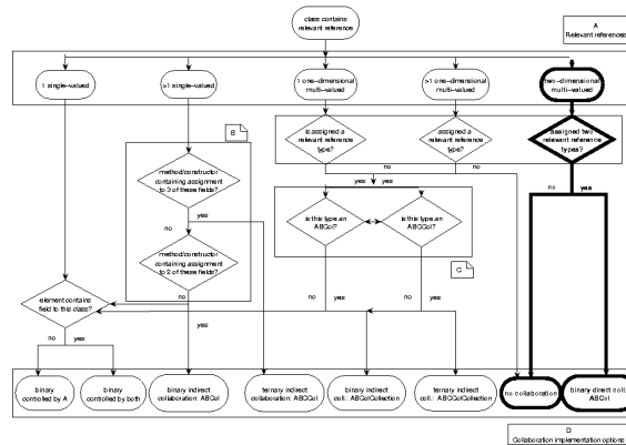
Figure 4.8: Collaboration detection for two-dimensional multi-valued fields
