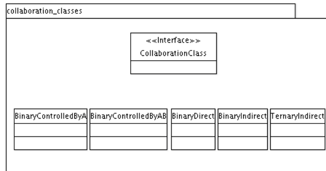
Figure 4.12: collaboration_classes package
