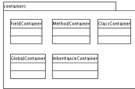
Figure 4.11: containers package
