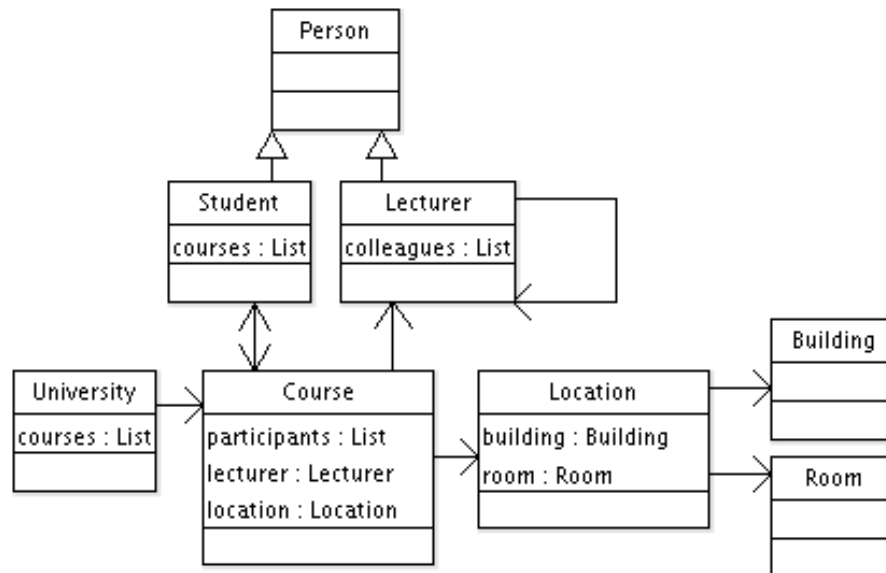
Figure 5.1: University example
