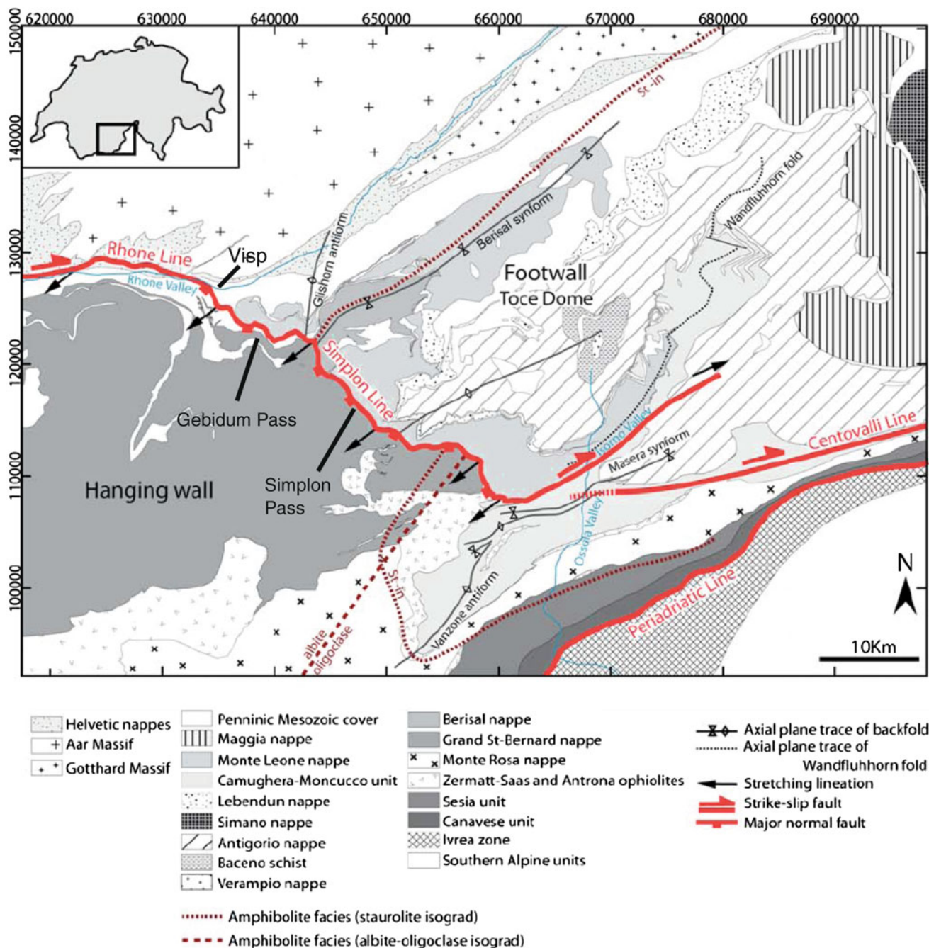
Fig. 2 Geological setting of the Simplon Fault Zone (SFZ) in the Central Alps, Switzerland. Geological map from Campani et al. (2010b) summarizing field observations of Campani et al. (2010a) and from published geological maps (Raron, Brig, Simplon,
