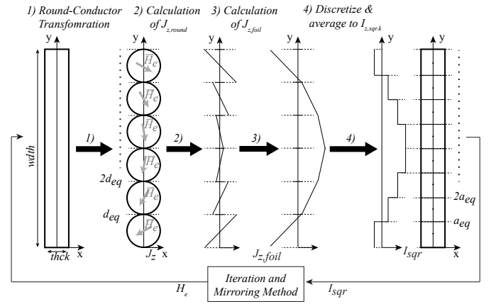
Figure 2. Overview calculation procedure for non-homogeneous current distribution in a foil, exposed to a 2-D transverse magnetic field: 1) Round-Conductor Transformation, 2) Calculation of round-conductor current density, 3) Calculation of foil current density, 4) Transformation to square-conductors and calculation of square-conductor currents.
