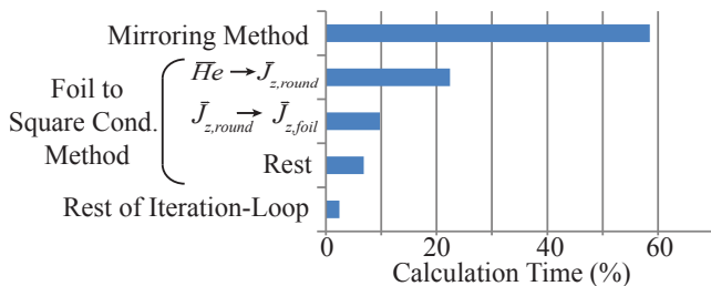
Figure 11. Flyback Transformer Model (specification as in table I at DC-DC BCM operation with harmonics from 100kHz to 2MHz): calculation complexity analysis with MATLAB profiler.
