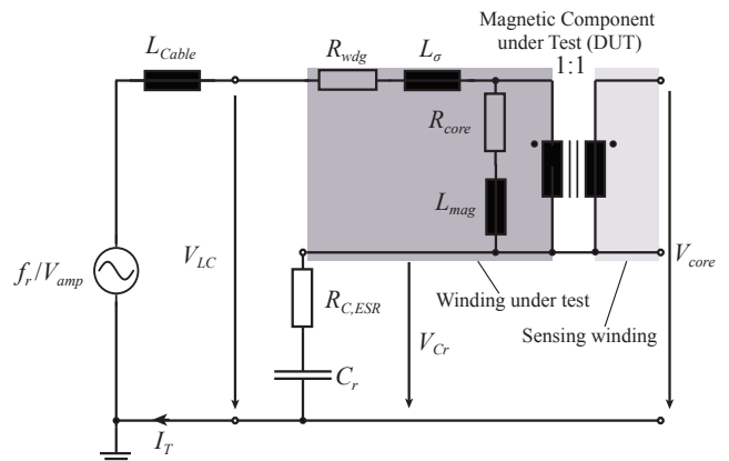
Figure 10. Overview measurement method for core- and winding-loss measurement of a magnetic component, according to [14].
