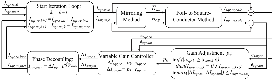
Figure 4. Overview numerical iteration for calculation of the non-homogeneous current distribution in foil windings.
