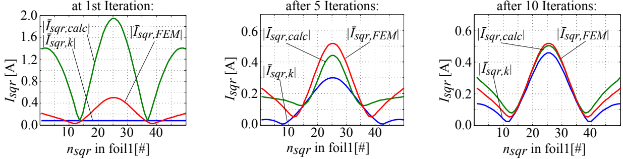
Figure 5. Numeric iteration for the current in foil 1 of the inductor with foil-winding (shown in fig. 1): \bar{I}_{sqr,k} and \bar{I}_{sqr,calc} at different iteration-steps in comparison to the current distribution \bar{I}_{sqr,FEM} derived from the 2-D FEM simulation of the inductor.
