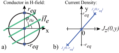
Figure 3. a) Round-conductor in a transverse H-field b) Linearized Eddy current density J_z in the round conductor evaluated on the y-axis: (0, -r_{eq}) , (0, 0) and (0, r_{eq}) .
