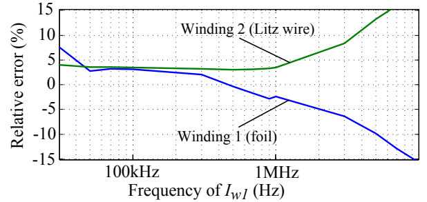
Figure 7. Flyback-Transformer as specified in tab. I, with sinusoidal excitation of the foil-winding ( I_{w1} = 5\text{A} ) and open circuit on the secondary: Relative difference between losses derived from the foil-to-square-conductor method and the 2D FEM simulation.
