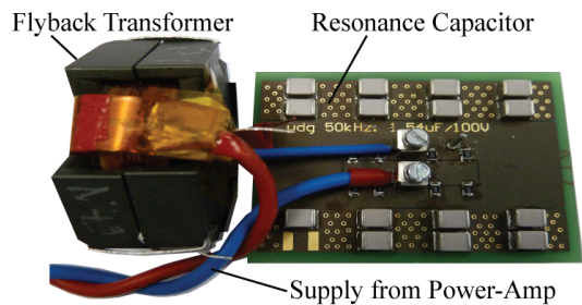
Figure 9. Experimental setup for winding loss measurement of the flyback transformer.
