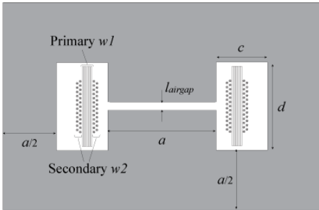
Figure 6. 2-D Flyback transformer with foils and Litz wires: E-core with air gap and 'sps' interleaved windings with foils on the primary and Litz wire for the secondary.
