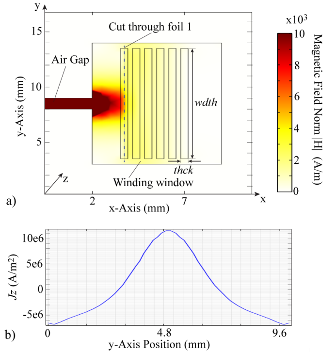
Figure 1. a) FEM Simulation with COMSOL: Foil windings in a winding window of a gapped magnetic core ( I_{foil}=5A/30kHz ) b) Non-homogeneous current density along foil 1 (see cut-line in fig.1a).The homogeneous current density would be 2.5e6A/m^2 .
